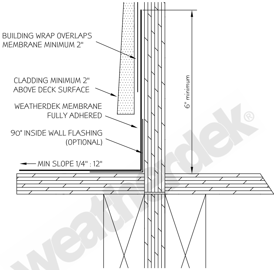
WD 11 WEATHERDEK INSIDE EDGE DETAIL TYPICAL INSIDE EDGE
