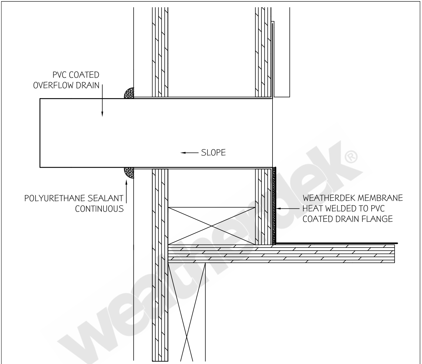
WD 24 WEATHERDEK PVC COATED OVERFLOW DRAIN DETAIL PVC COATED OVERFLOW DRAIN
