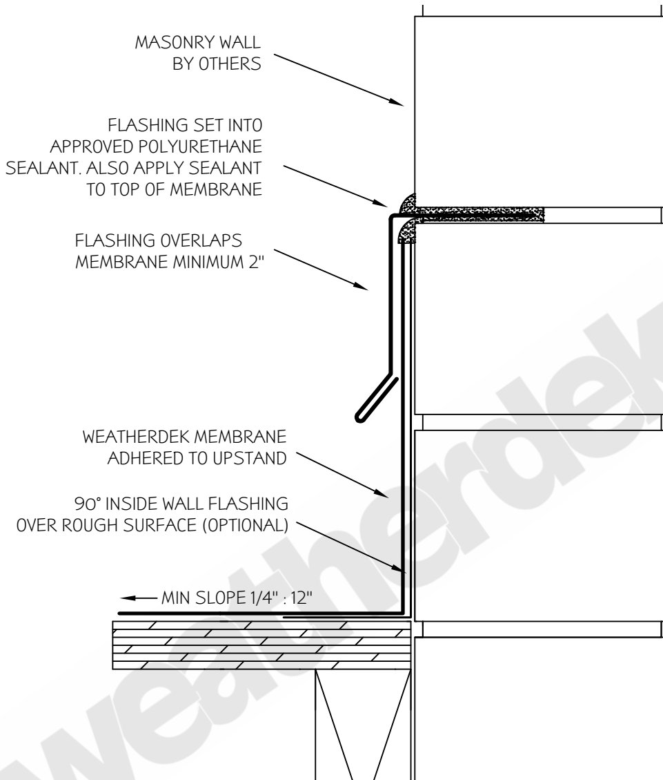
WEATHERDEK MASONRY INSIDE EDGE DETAIL TYPICAL INSIDE EDGE
