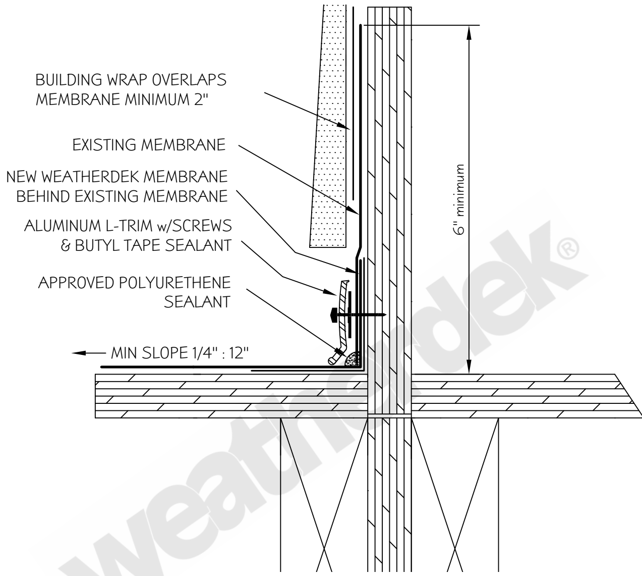
WD 14 WEATHERDEK TIE IN TO EXISTING MEMBRANE TYPICAL INSIDE EDGE
