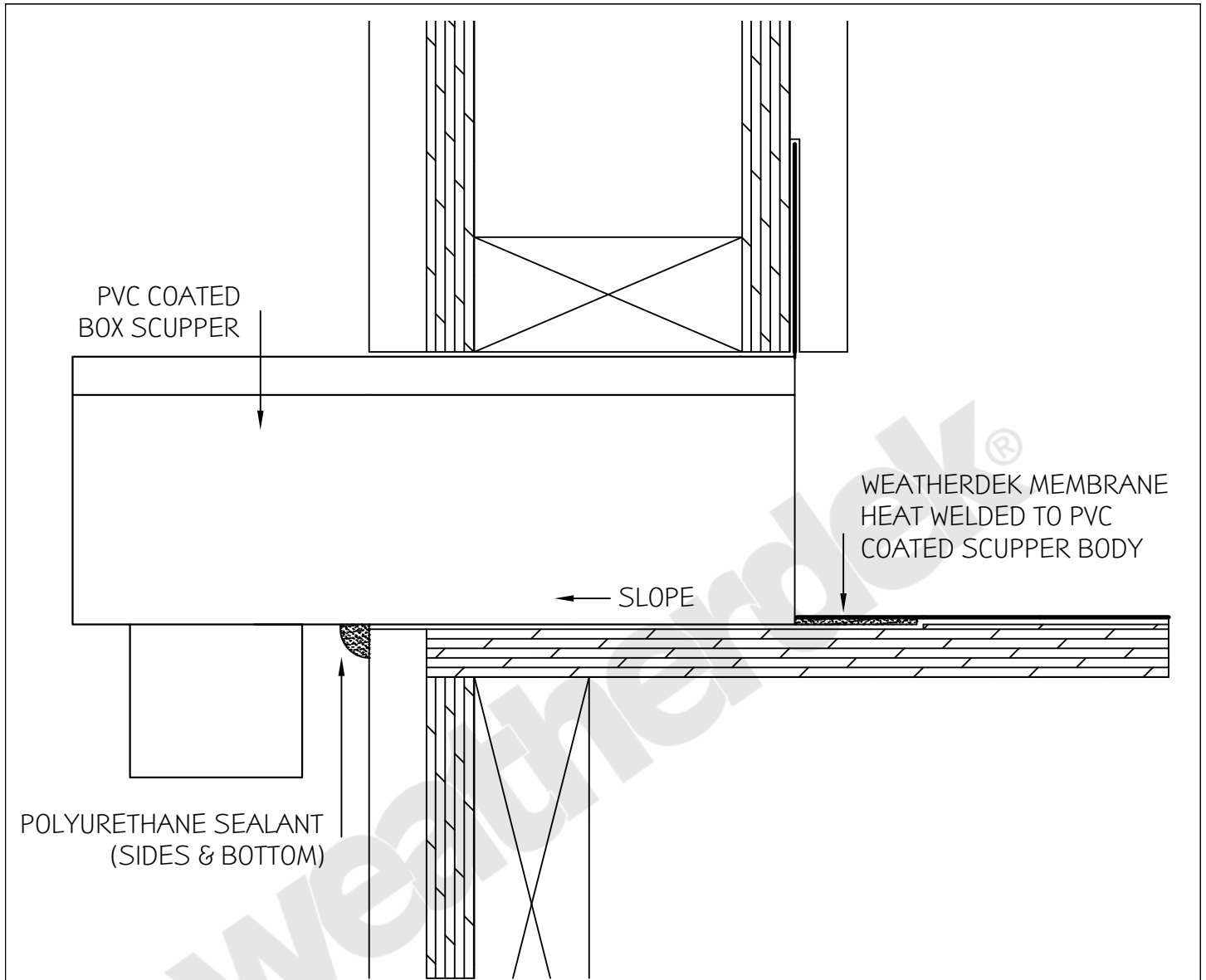
WEATHERDEK PVC COATED SCUPPER DETAIL PVC COATED BOX SCUPPER
