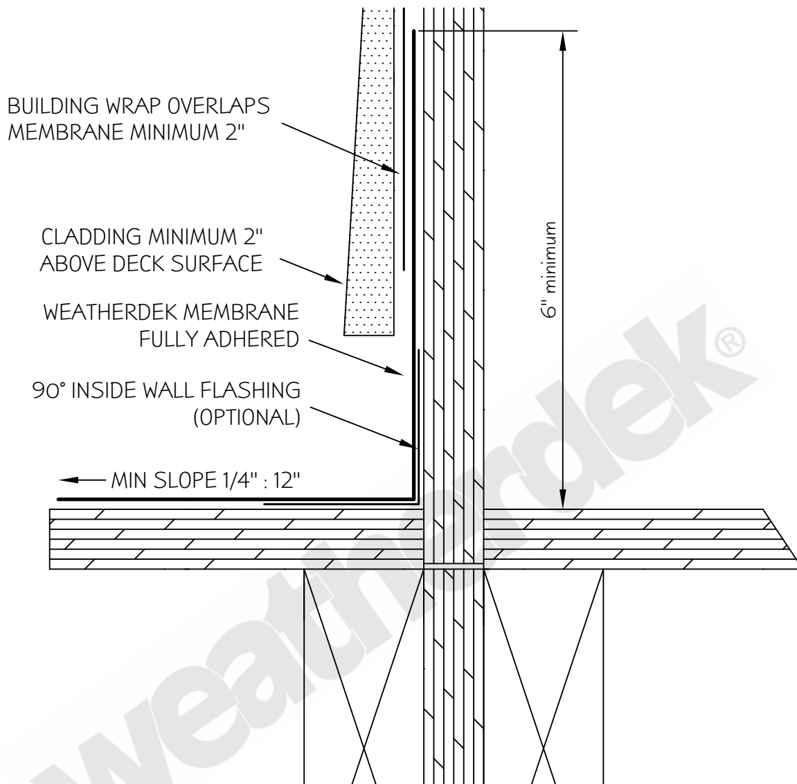
WEATHERDEK INSIDE EDGE DETAIL TYPICAL INSIDE EDGE
