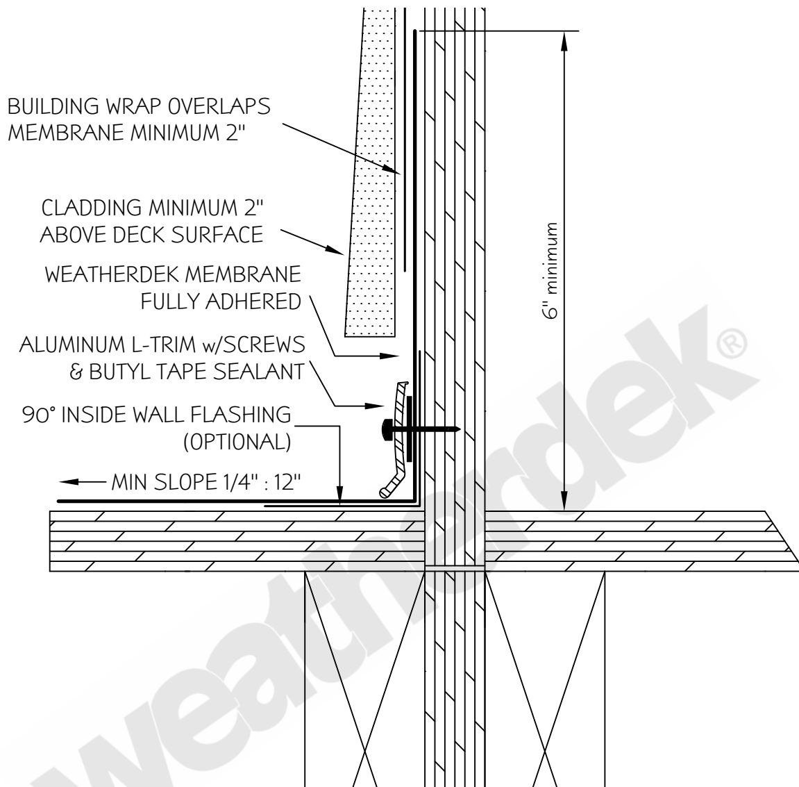
WEATHERDEK INSIDE EDGE 'L-TRIM' DETAIL TYPICAL INSIDE EDGE
