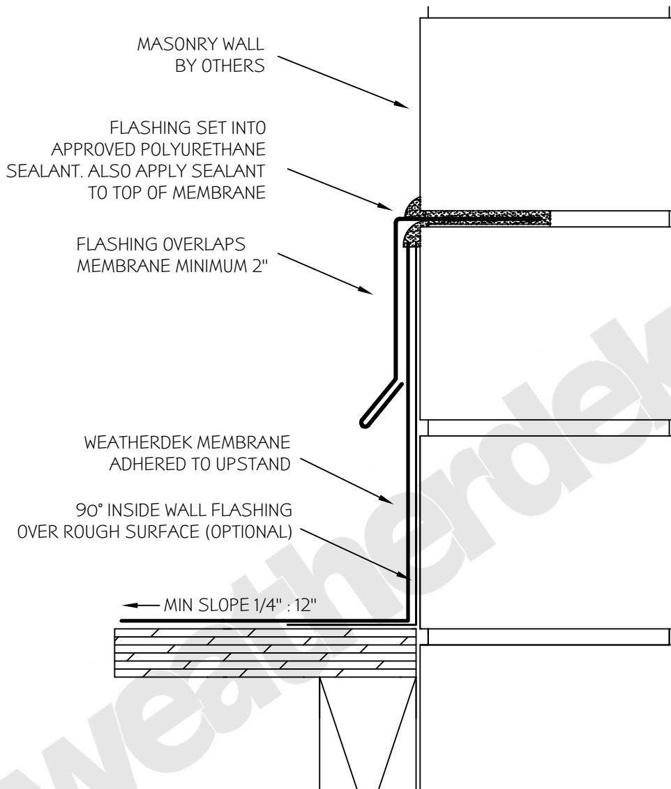
WD 13 WEATHERDEK MASONRY INSIDE EDGE DETAIL TYPICAL INSIDE EDGE
