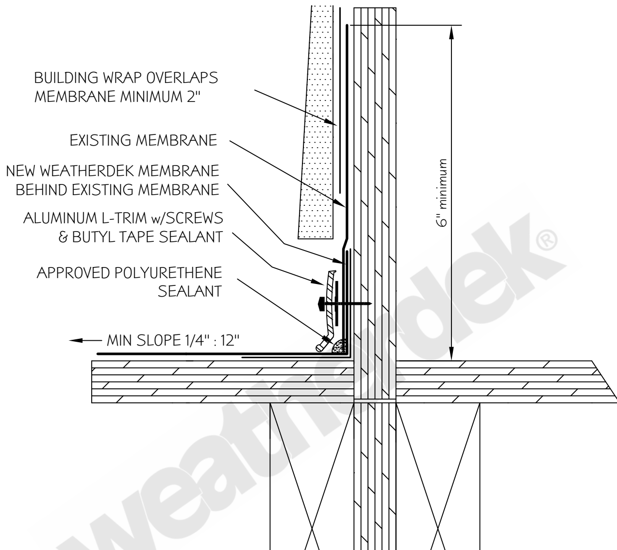
WEATHERDEK TIE IN TO EXISTING MEMBRANE TYPICAL INSIDE EDGE
