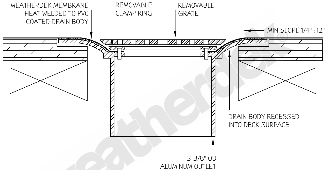
WD 22 WEATHERDEK PVC COATED DRAIN DETAIL PVC COATED ALUMINUM DRAIN
