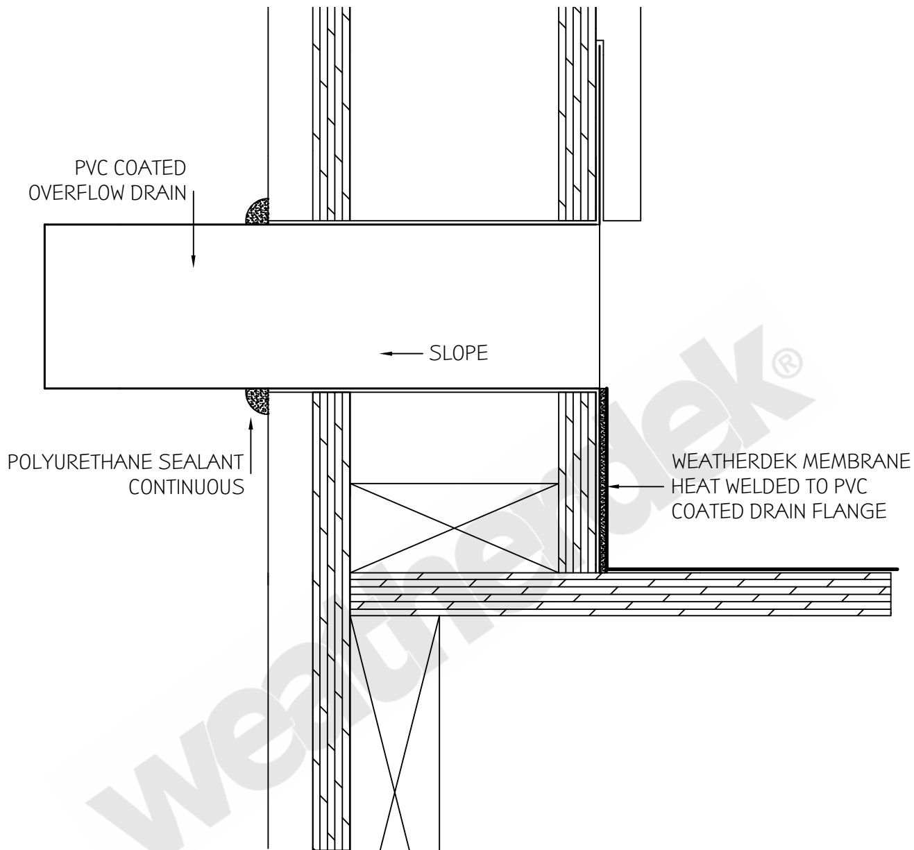
WEATHERDEK PVC COATED OVERFLOW DRAIN DETAIL PVC COATED OVERFLOW DRAIN
